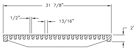
GRATE SECTION
