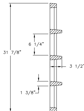
GRATE SECTION
